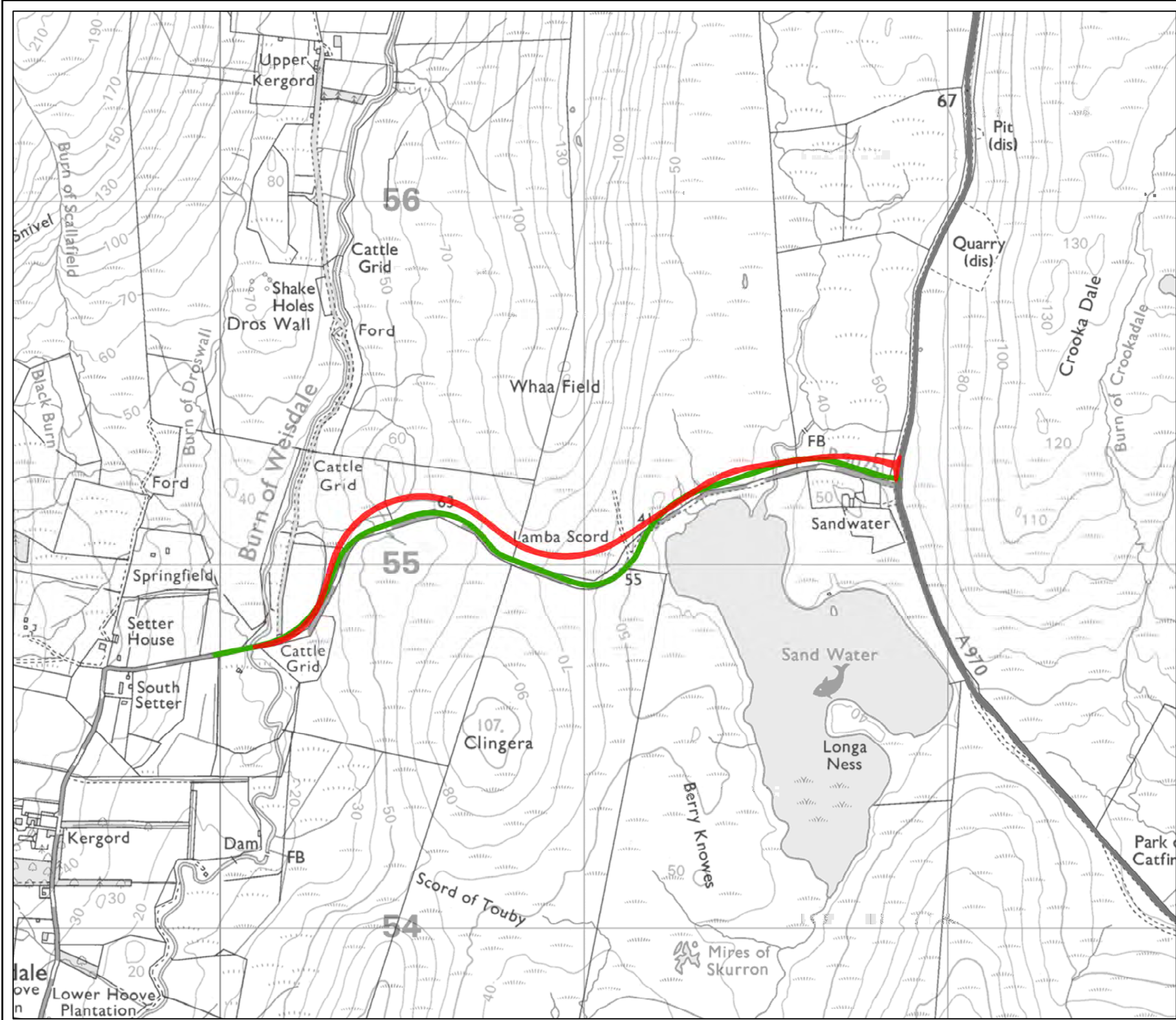
Figure 3.1 Comparison Showing 2016 and 2019 Alignment B9075 Sandwater Road Realignment EIA Report
